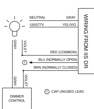
FIGURE 2 - IIS 550 I DIMMING RELAY CONNECTIONS (SEE FIGURE 2 FOR COMPLETE WIRING INSTRUCTIONS)
