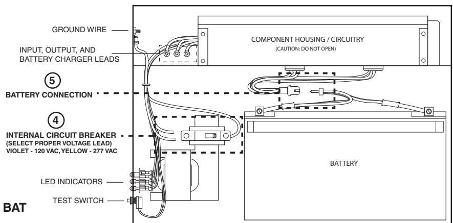
FIGURE 3 - IIS 550 I SIDE
