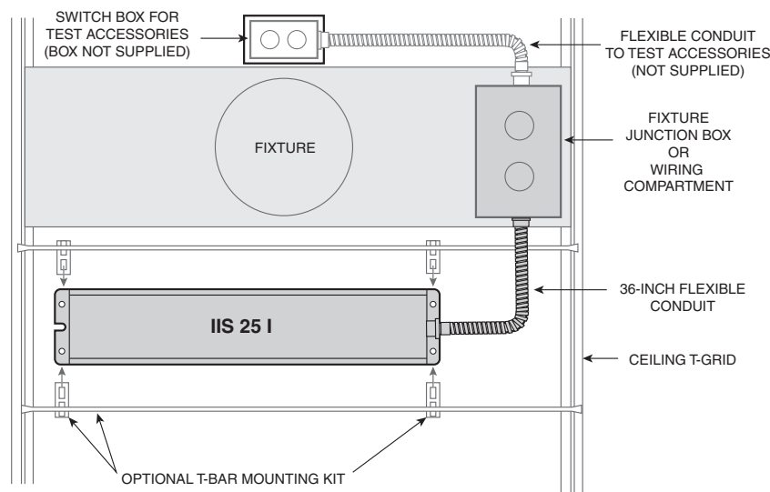
Illustration 1: IIS 25 I and Test Accessory Mounting (Top View)
