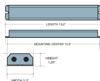
ILB CP10 B: 13.0" x 2.2" x 1.25" (mounting center 12.6")
