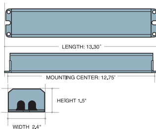
ILB CP10 A: 13.3" x 2.375" x 1.5" (mounting center 12.75")
