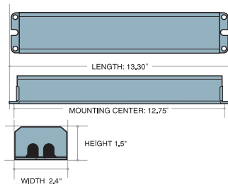
ILB CP12 A: 13.3" x 2.375" x 1.5" (mounting center 12.75")
