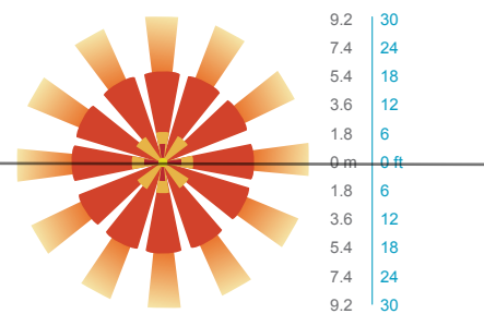
15 FT MOUNTING
