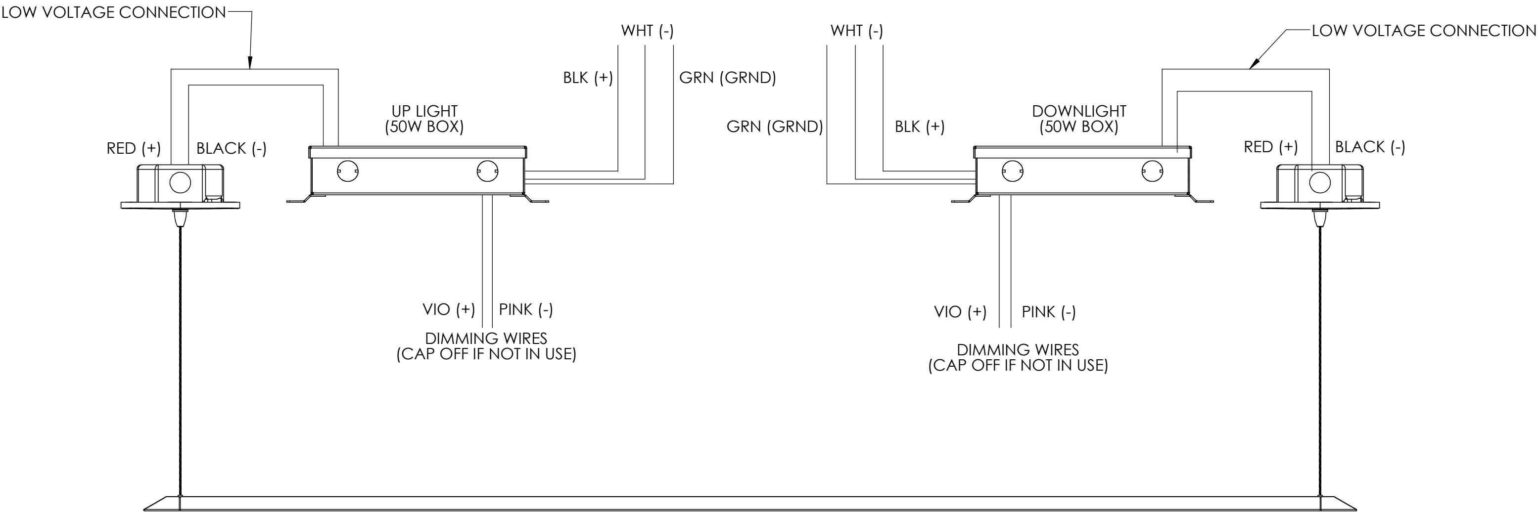
4FT INDIVIDUAL FIXTURE
