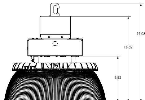
WHK Mounting (IE20WCPHE or IE30WCPHE options) Top Battery Box
