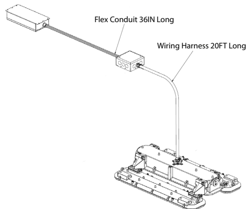
12000LM-30000LM FIXED WITH REMOTE EM BATTERY (IE20WCPHER or IE30CPHER)
