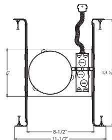
5 5/8" CEILING CUTOUT
