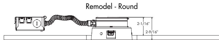
5 5/8" CEILING CUTOUT
