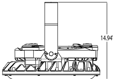
HOL01 HA Yoke Mount (YK90 - Large Electrical)
