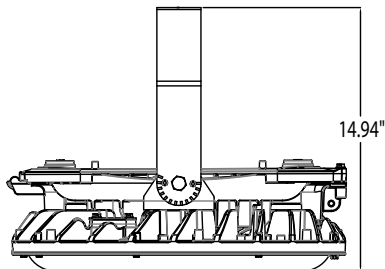
HOL01 Yoke Mount (YK90 - Small Electrical)
