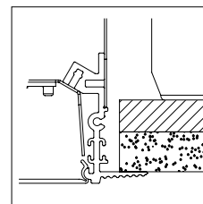
GBNB Gypsum Board (sheetrock) Install From Below
