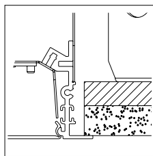
FLNB 5/8IN Flange (sheetrock) Install From Below
