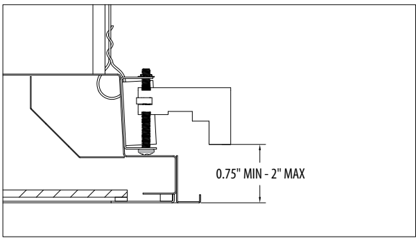
2X2 with Sensor, Inset Door Frame
