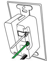
STEP 3 Connect Neutral to Silver Screw & Ground to Green Screw
