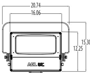
YK-Yoke Mount Luminaire EPA of 1.76 Ft 2 and max weight 31 lbs.
