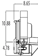
YK-Yoke Mount Luminaire EPA of 1.76 Ft 2 and max weight 31 lbs.
