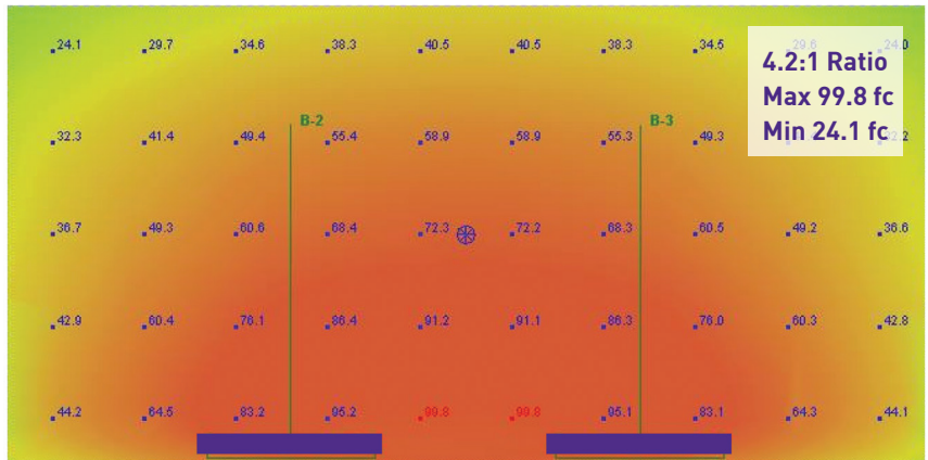
Two 2' Hydrel 4750 (8000 Lumens)
