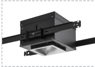
EVO square MRI downlight (Series: EVO4SQM, EVO6SQM) / lm/W: Up to 106.9
